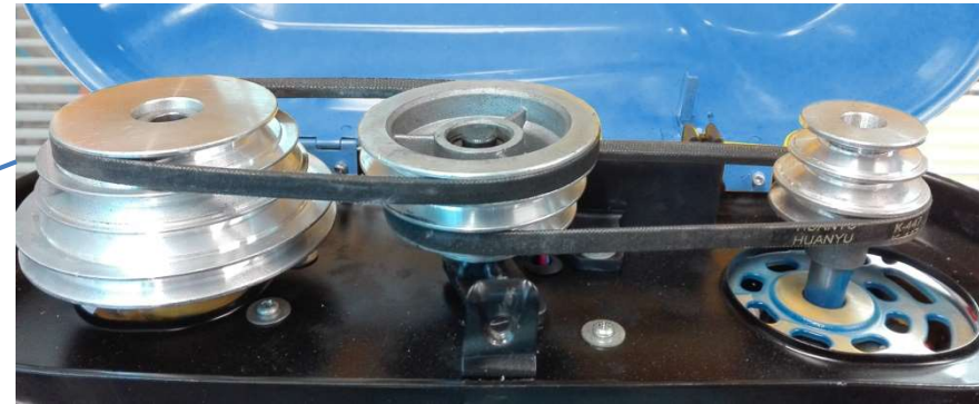
Transmission system with three pulleys and double belt
