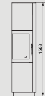
Speicherstein-Thermoblock
