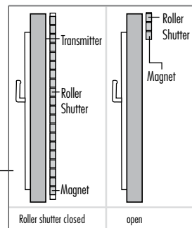
Positioning Roller Shutter Transmitter (side view)
